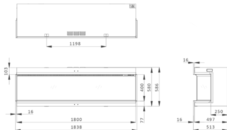
Trimline iX18
