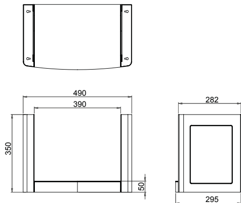
Pedestal
