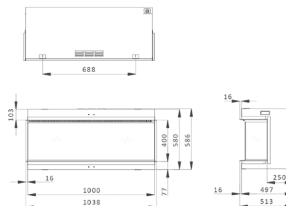
Trimline iX10
