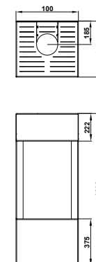
Trimline 38 FS Mantel
