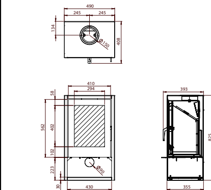
Woodfire Cubic 6kW
