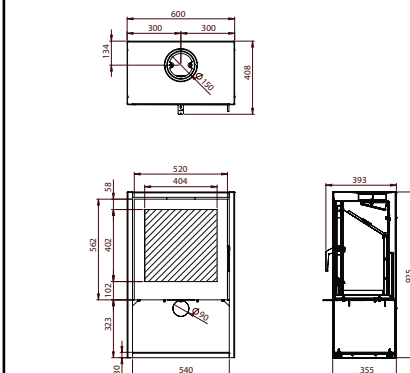
Woodfire Cubic 8kW
