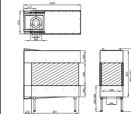
Trimline 85 Room divider
